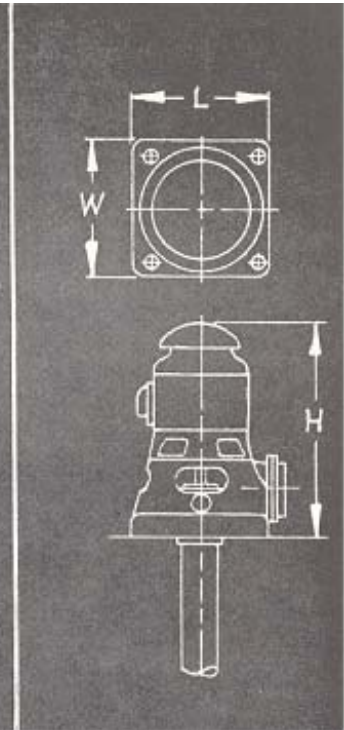
Figure 3. VERTICAL turbine pump
