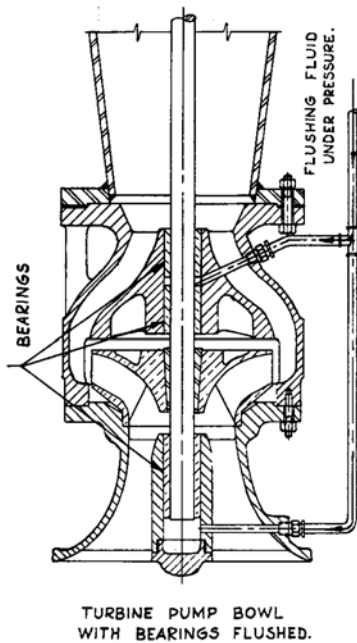
Figure 5. Vertical Pump bowl designed for use of special flushing fluid.
