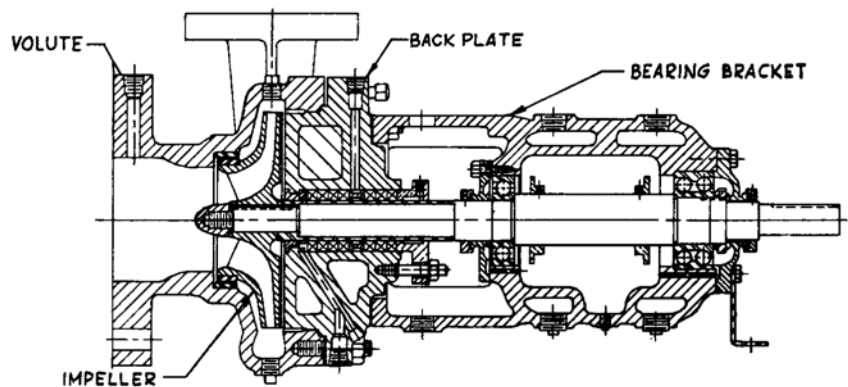
Figure 6. Typical horizontal process pump.
