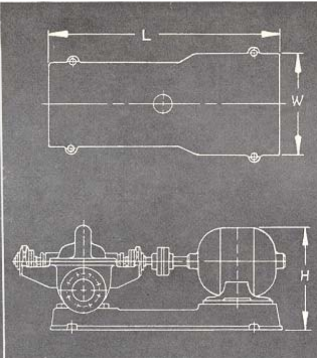
Figure 2. HORIZONTAL double suction split case.
